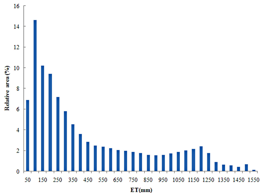
Figure 4. Frequency distribution of the ETLook estimated annual ET in the Indus Basin at spatial resolution of 1 km \times 1 km for 2007.
