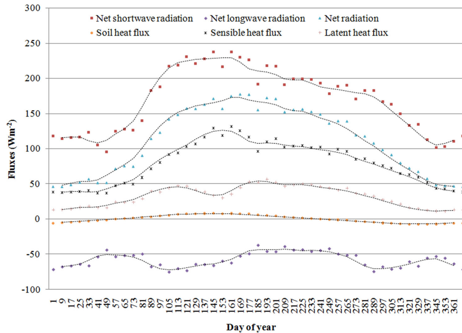
Figure 2. Temporal variation of components of the surface energy equation during 2007 in the entire Indus Basin (116.2 mha). The dashed lines represent 24 days moving average values.
