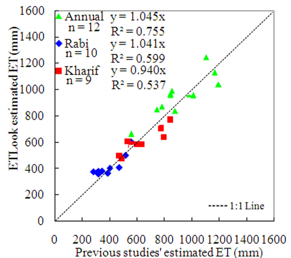
Figure 7. Comparison of evapotranspiration modeled/estimated by previous studies conducted during the years 1995–1996 [Bastiaansen et al. , 1999], 2000 [Sarwar and Bill, 2007], 2001–2002 [Ahmad et al. , 2009; Shakoore et al. , 2006] and 1999–2006 [Shakir et al. , 2010] and ET estimated by ETLook for 2007 in the Indus Basin.
